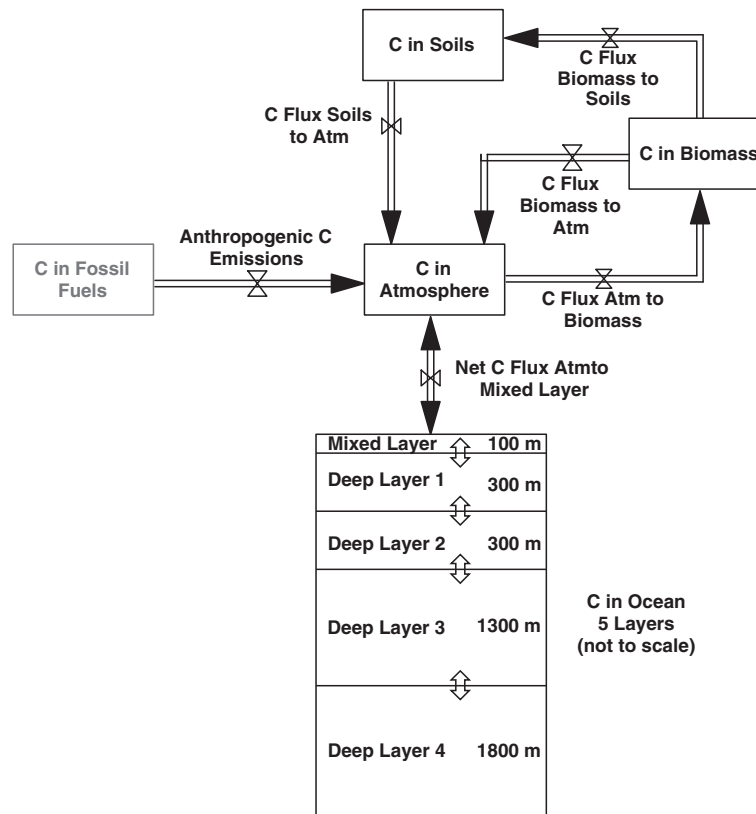
Fig. 2. C-ROADS carbon cycle. Stocks of C in fossil fuels not treated explicitly. CH 4 fluxes and atmospheric stock and C fluxes and stocks due to deforestation/afforestation are represented explicitly but are aggregated in this simplified view
