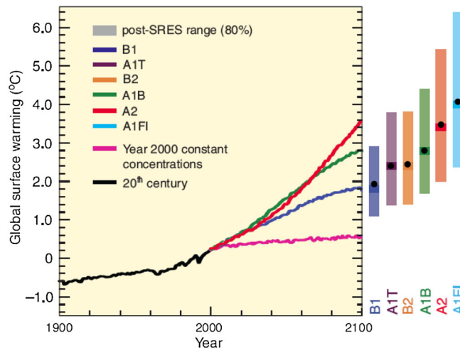
Fig. 4. Temperature projections for 2100 and likely range from IPCC AR4 (SPM, Figure 5) vs. C-ROADS (black circles)
