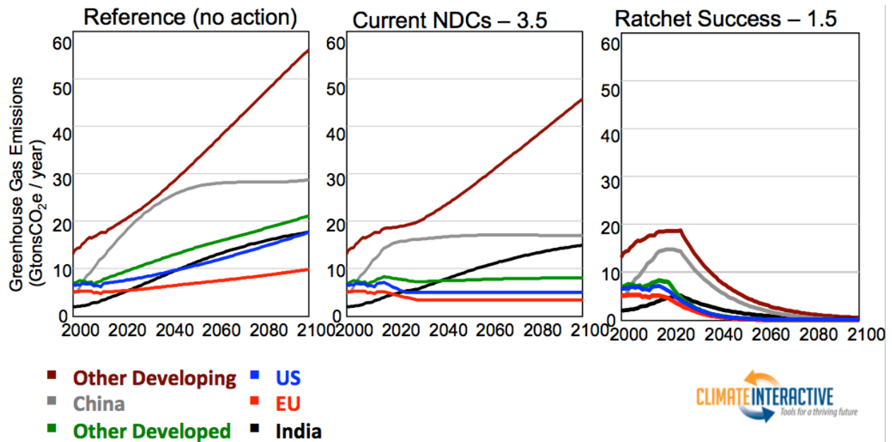
Figure 3: Greenhouse gas emissions from 2000-2100 for six regions of the world, under three scenarios.
